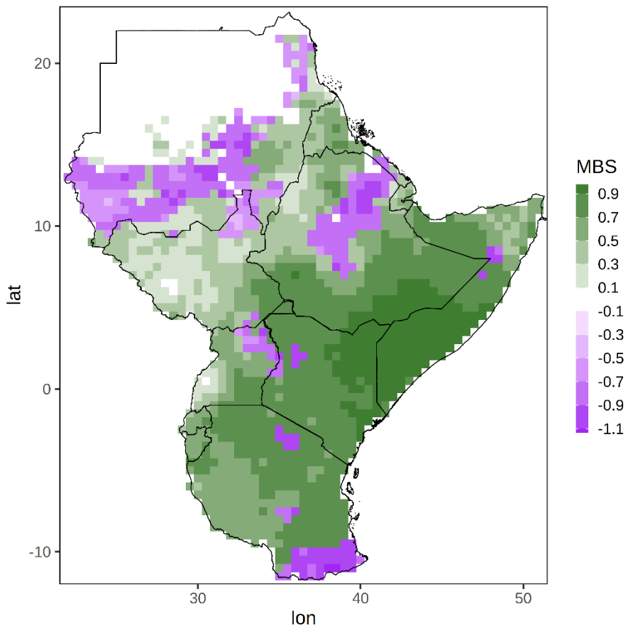
MBSS for OND tercile forecast 2023
