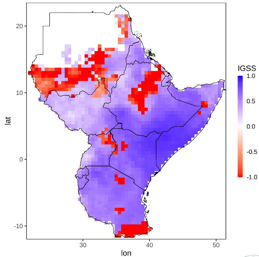
IGSS for OND tercile forecast 2023
