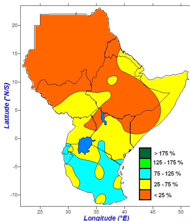
Figure 4: Spatial pattern of rainfall anomalies for December 2014 to February 2015 period
