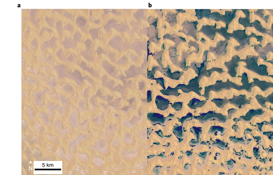
Fig. 1 | Desert lakes in the 'Empty Quarter'. Pools of water form in Rub' al-Khali desert, also known as the 'Empty Quarter', due to intense rainfall under tropical cyclone Mekunu. a , Photograph taken on 13 May 2018 shows normal dry conditions. b , Photograph taken on 29 May 2018 shows the 'desert lakes' that facilitate locust breeding and survival. NASA Earth Observatory images by L. Dauphin using US Geological Survey data.
