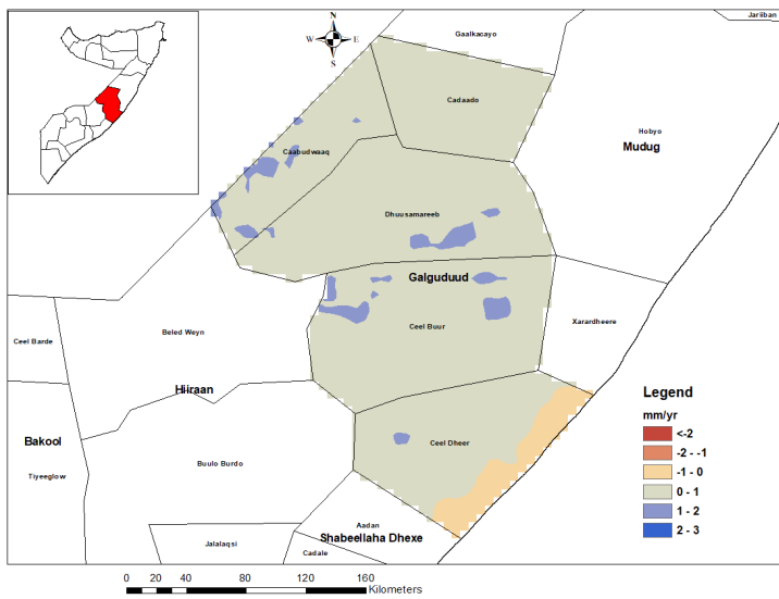
Figure 6: SON Season Rainfall Trend/Yr (1981-2018)
