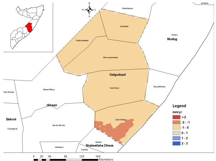
Figure 5: MAMJ Season Rainfall Trend/Yr (1981-2018)
