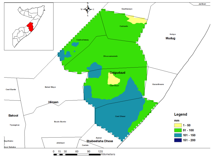
Figure 4: SOND Long Term Mean Rainfall (1981-2010)
