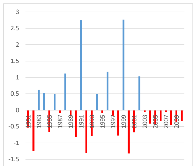
Figure 3.3-2 Rainfall anomaly in Sept to Dec (1981–2010), Somaliland
