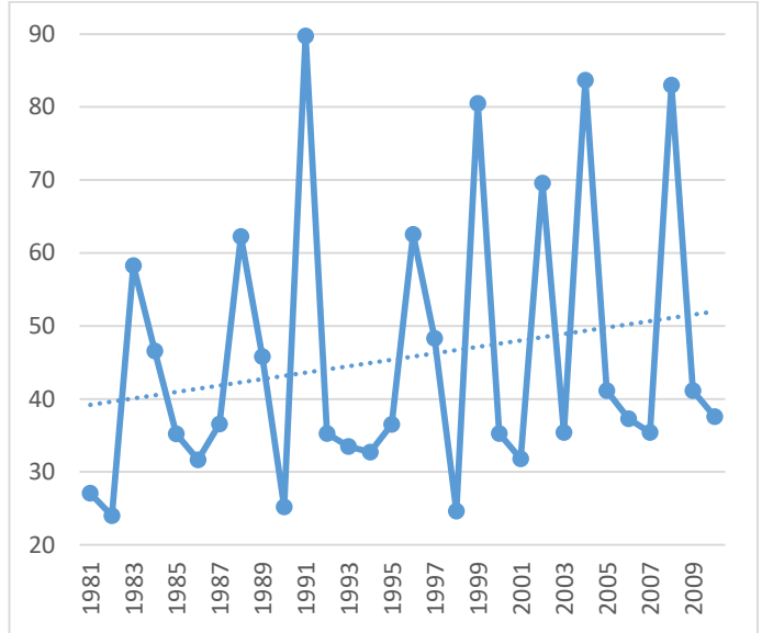
Figure 3.4-4 SOND Rainfall totals in Sept to Dec Season at the Puntland site
