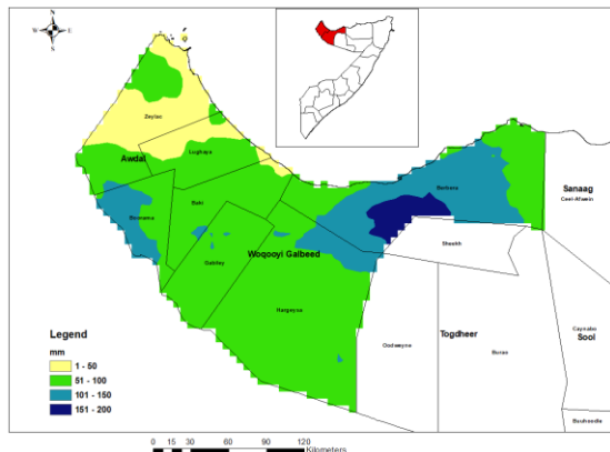
Figure 3.2-7 Sept – Dec (SOND) seasonal rainfall (1981-2010), Somaliland
