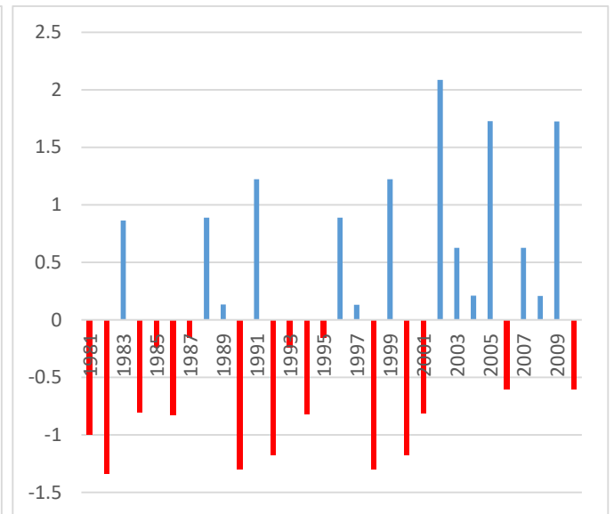
Figure 3.3-6 Rainfall anomaly in Sept to Dec (1981–2010), Galmudug
