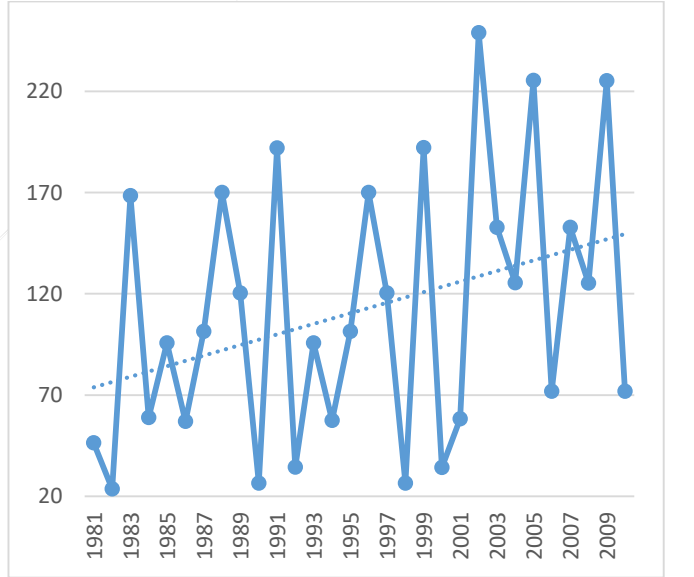
Figure 3.4-6 SOND Rainfall totals in Sept to Dec Season at the Galmudug site
