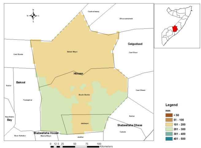
Figure 3.1-12 Annual minimum rainfall extremes 1981-2010 Hirshabelle
