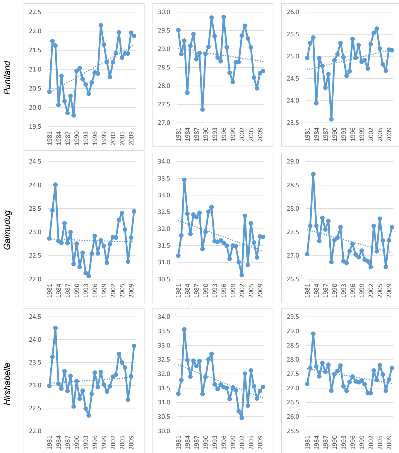
Figure 3.11-11 Time series for minimum, maximum and average temperature for RLACC sites (1981-2010)
