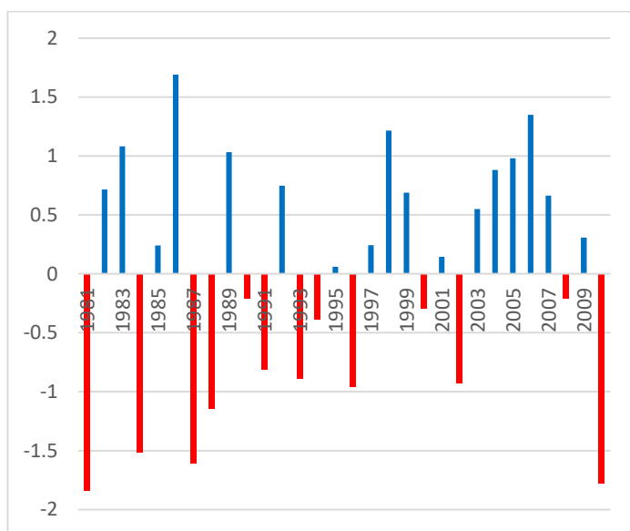
Figure 3.3-1 Rainfall anomaly in March to June (1981–2010), Somaliland
