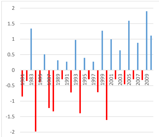
Figure 3.3-3 Rainfall anomaly in March to June (1981–2010), Puntland
