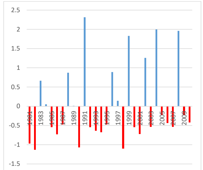
Figure 3.3-4 Rainfall anomaly in Sept to Dec (1981–2010), Puntland
