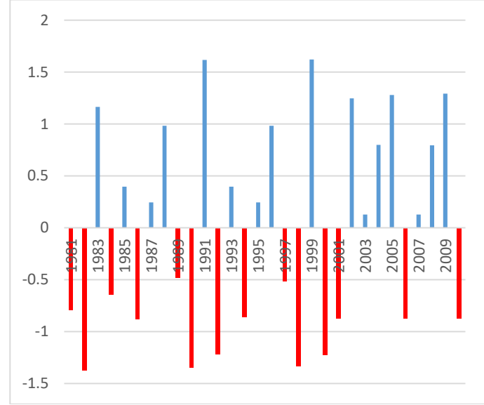
Figure 3.3-8 Rainfall anomaly in Sept to Dec (1981–2010), Hirshabelle
