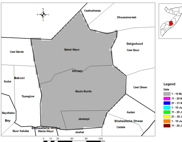
Figure 3.10-17 Historical cessation in the Gu Season (1981-2018) at the Hirshabelle site
