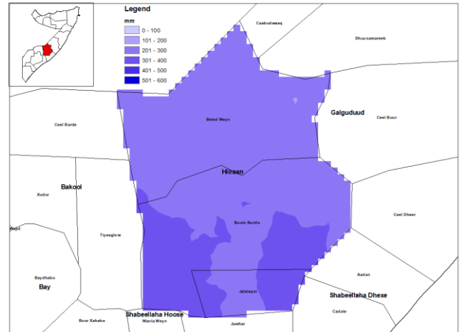
Figure 3.1-4 Mean annual rainfall 1981-2010 Hirshabelle
