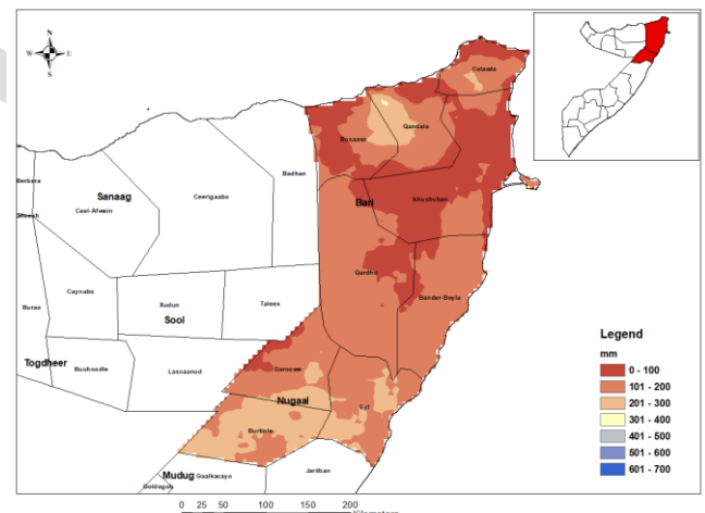
Figure 3.1-6 Annual maximum rainfall extremes 1981-2010 Bari and Nugal, Puntland
