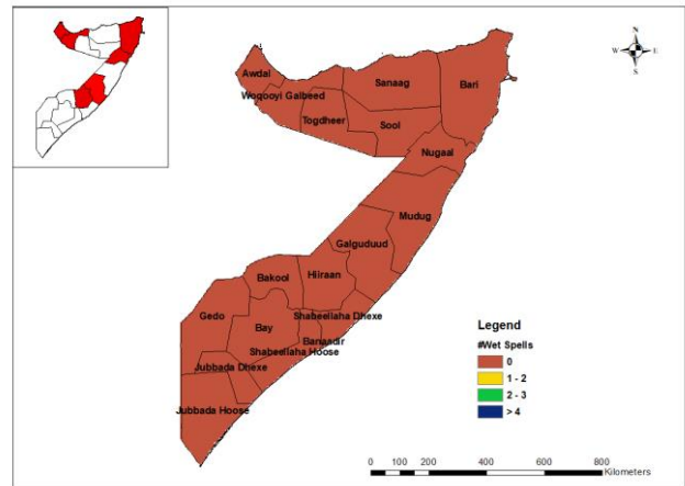
Figure 3.7-1 Number of wet spells in MAMJ in Somalia Figure 3.7-2: Number of wet spells in SOND in Somalia
