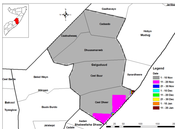
Figure 3.10-16 Historical cessation in the Deyr Season (1981-2018) at the Galmudug site
