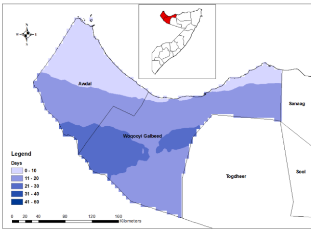
Figure 3.6-1 Average Number of Wet days in the (MAMJ) Season (1981-2010) at the Somaliland site
