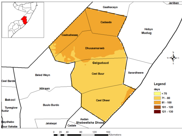
Figure 3.8-5 Average Number of dry days in the (MAMJ) Season (1981-2010) at the Galmudug site
