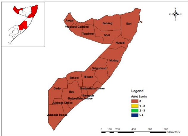
Figure 3.7-1 Number of wet spells in MAMJ in Somalia Figure 3.7-2: Number of wet spells in SOND in Somalia
