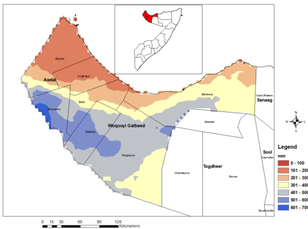
Figure 3.1-5 Annual maximum rainfall extremes 1981-2010 Awdal and Woqooyi Galbeed, Somaliland
