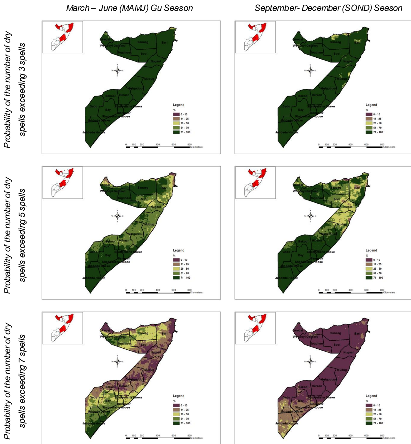
Figure 3.9-11 Probability of the number of dry spells in the MAMJ & SOND season exceeding 3, 5 and 7 dry spells
