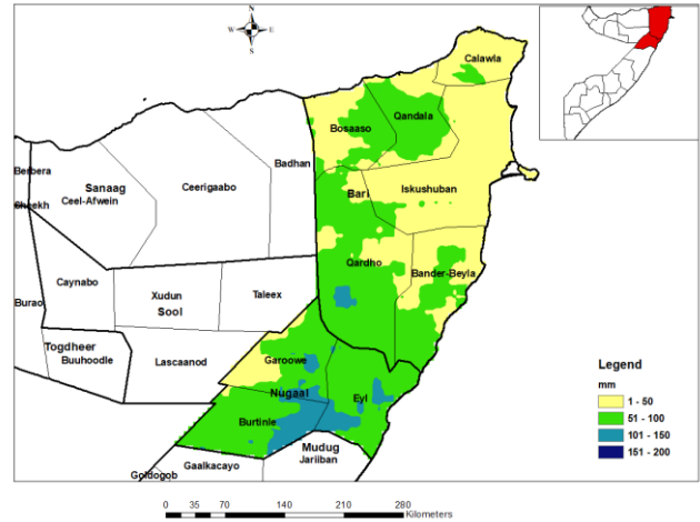
Figure 3.2-4 March – June (AMJ) seasonal rainfall (1981-2010), Puntland
