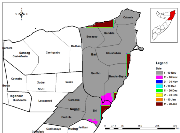
Figure 3.10-14 Historical cessation in the Deyr Season (1981-2018) at the Puntland site
