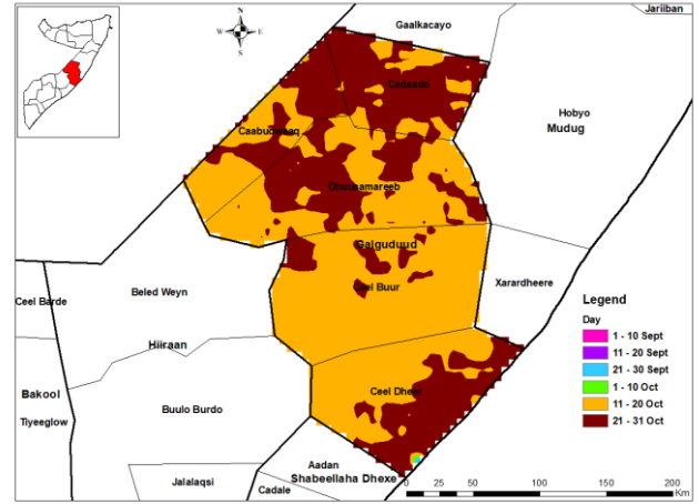
Figure 3.10-6 Historical onset in the Deyr Season (1981-2018) at the Galmudug
