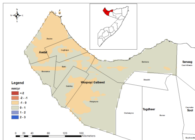
Figure 3.4-12 SOND Trend per year in Sept to Dec Season at the Somaliland site
