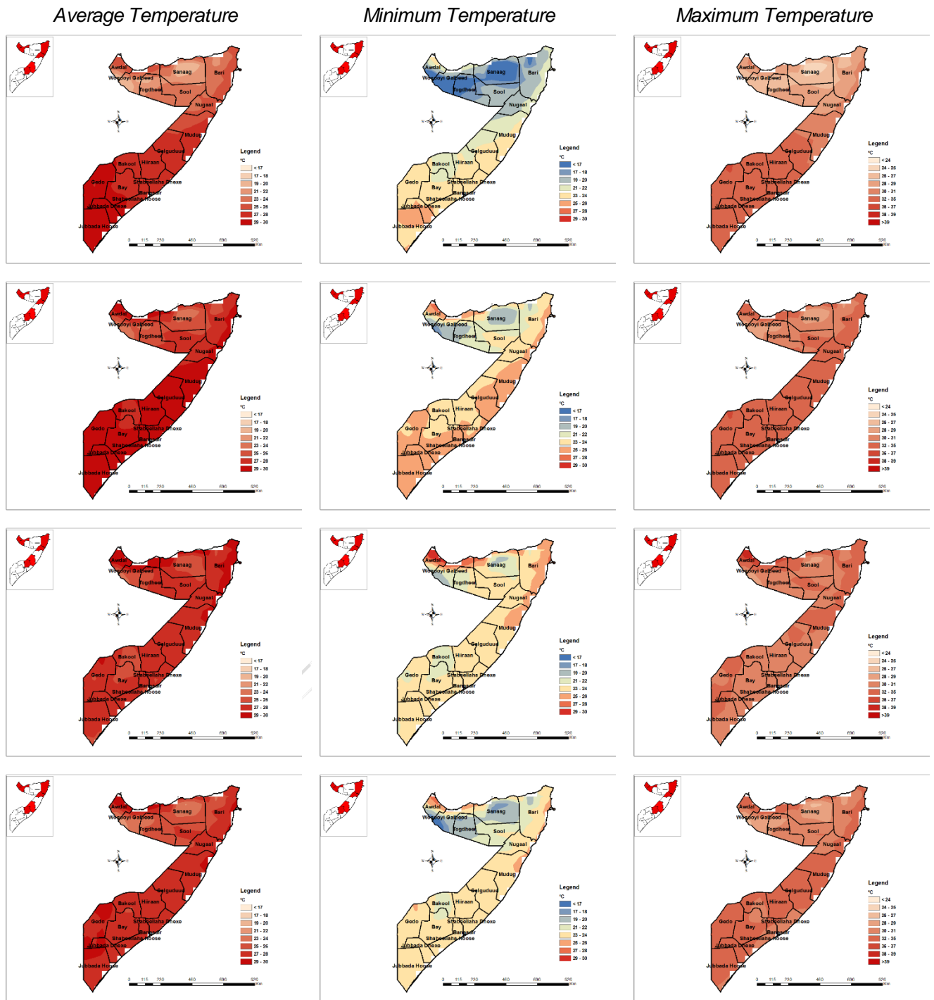
Figure 3.11-10 Average Seasonal Temperature over Somalia (1981-2010)
