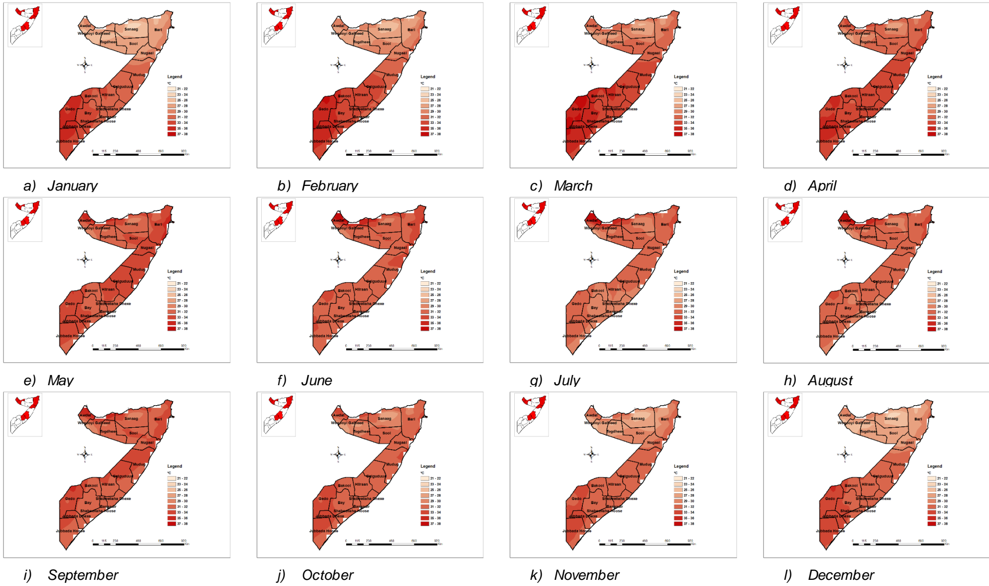
Figure 3.11-9 Average Monthly Maximum Temperature over the Somalia Region (1981-2010)
