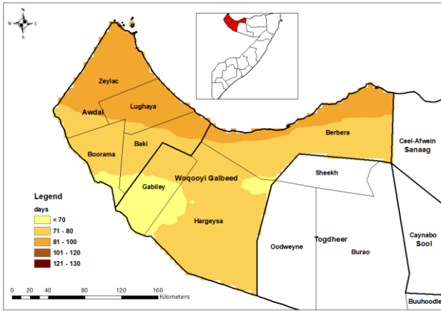
Figure 3.8-1 Average Number of dry days in the (MAMJ) Season (1981-2010) at the Somaliland site
