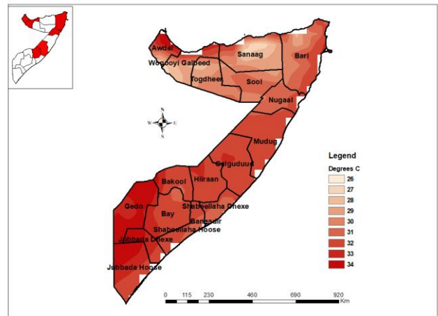
Figure 3.11-3 Mean annual maximum surface temperature climatology (1981–2010) for the Somalia region
