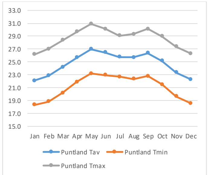
Figure 3.11-5 Minimum, Maximum and Average Monthly Temperature over Project Site in Puntland (1981-2010)
