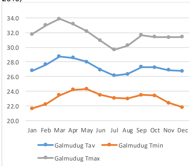
Figure 3.11-6 Minimum, Maximum and Average Monthly Temperature over Project Site in Galmudug (1981-2010)
