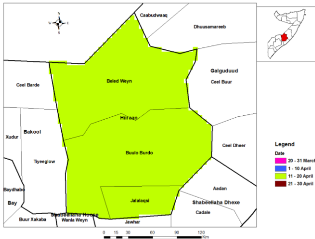
Figure 3.10-7 Historical onset in the Gu Season (1981-2019) at sites in Hirshabelle
