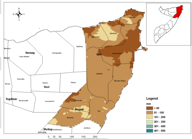
Figure 3.1-10 Annual minimum rainfall extremes 1981-2010 Bari and Nugaal, Puntland
