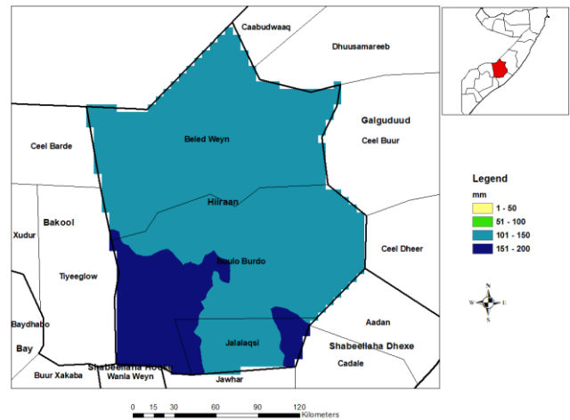
Figure 3.2-6 April – June (AMJ) seasonal rainfall (1981-2010), Hirshabelle
