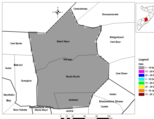
Figure 3.10-18 Historical cessation in the Deyr Season (1981-2018) at the Hirshabelle site
