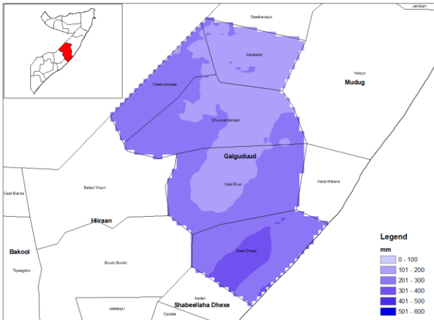
Figure 3.1-3 Mean annual rainfall 1981-2010 Galmudug
