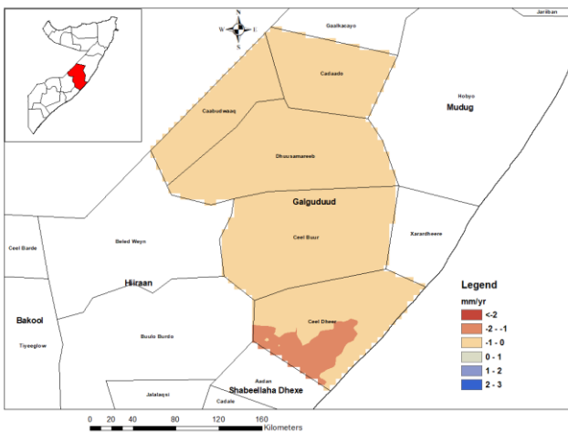
Figure 3.4-15 MAMJ Trend per year in March to June Season at the Galmudug site
