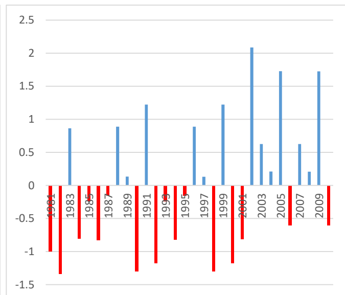
Figure 3.3-6 Rainfall anomaly in Sept to Dec (1981–2010), Galmudug
