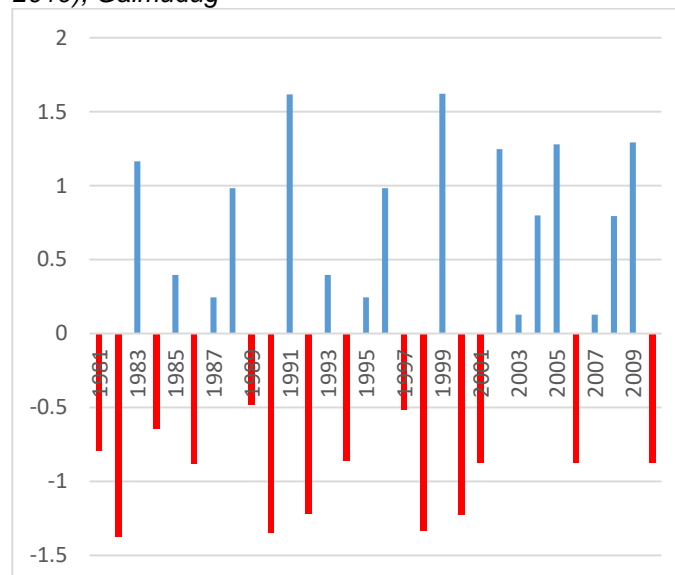
Figure 3.3-8 Rainfall anomaly in Sept to Dec (1981–2010), Hirshabelle
