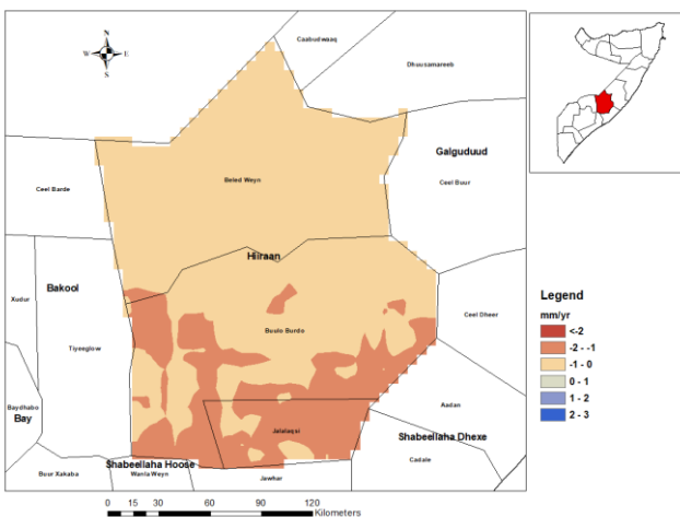
Figure 3.4-17 MAMJ Trend per year in March to June Season at the Hirshabelle site
