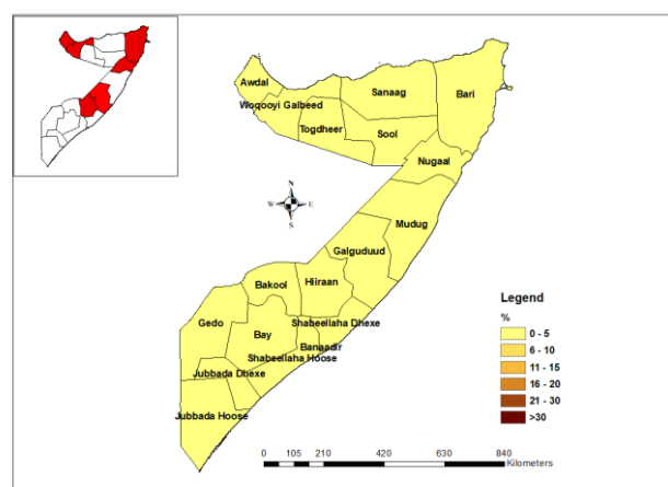
Figure 3.5-18 Probability of Rainfall intensity exceeding 5 mm a day Deyr (SOND) (1981-2010) in Somalia
